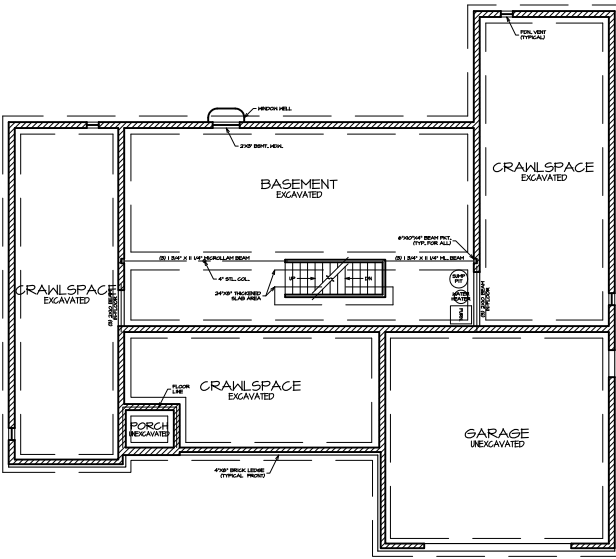
FOUNDATION PLAN
